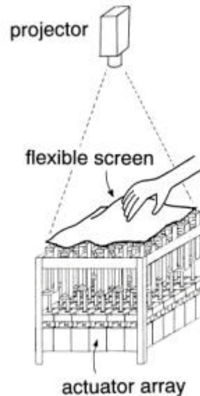
Figure 1. Basic idea of the FEELEX
