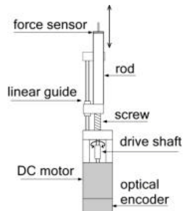
Figure 3. Linear actuator
